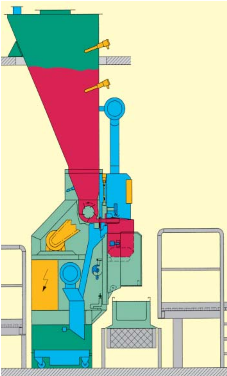
Cross-sectional view of a HAYER valve-bag filling machine with the vertical impeller filling system and automatic, vertical bag discharge
