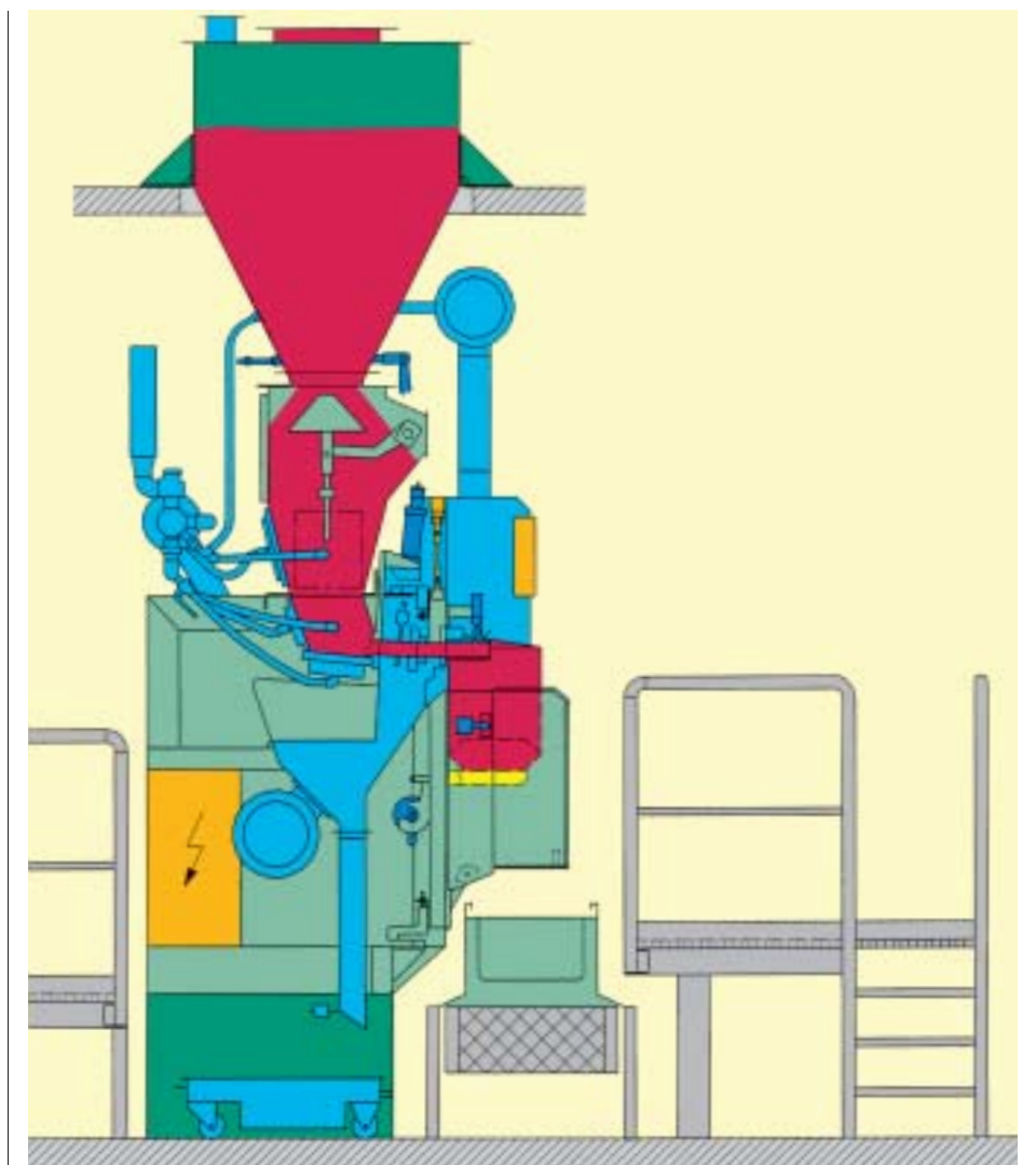
Cross-sectional view of a HAYER valve-bag filling machine using the air entrainment system
