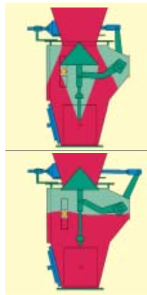
Cone valve (opened / closed)
